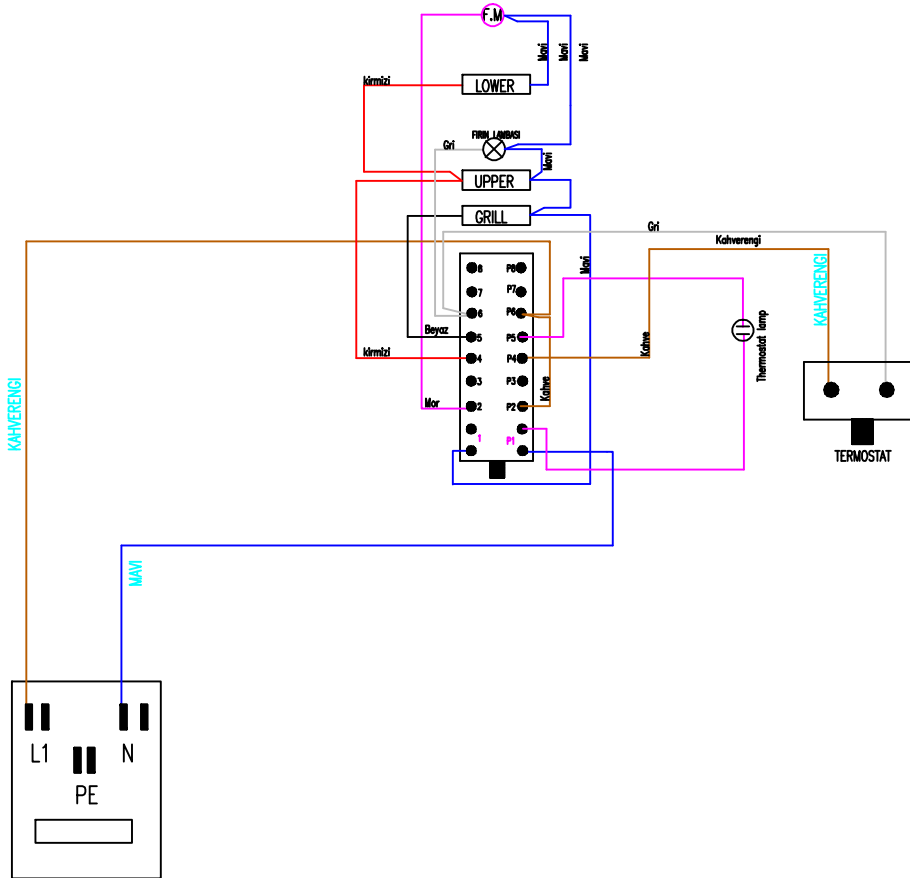
TERMINAL BOX
